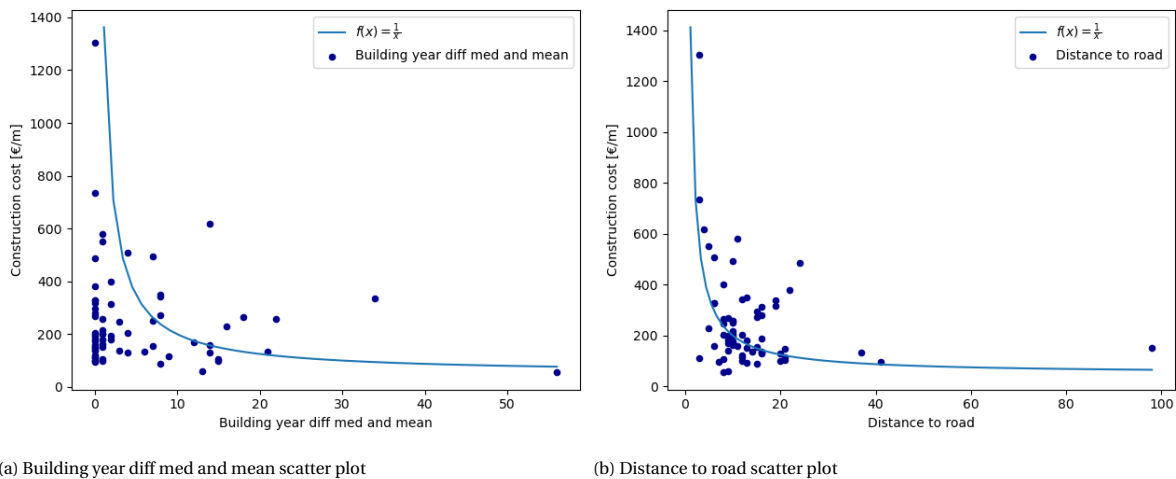
Figure 6.2: Scatter plots non-linear input parameters water
